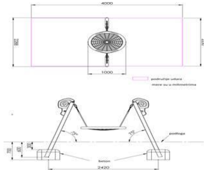
Скица 1. Љуљашка - Swing BABY SNAIL (with seat BIRD NEST)
